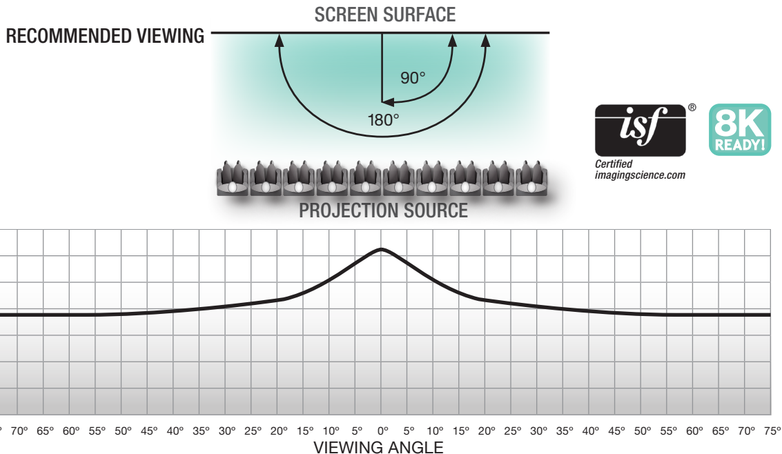
GAIN CHART TECVISION XT1600X WHITE
